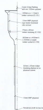
FASCIA PROFILE
