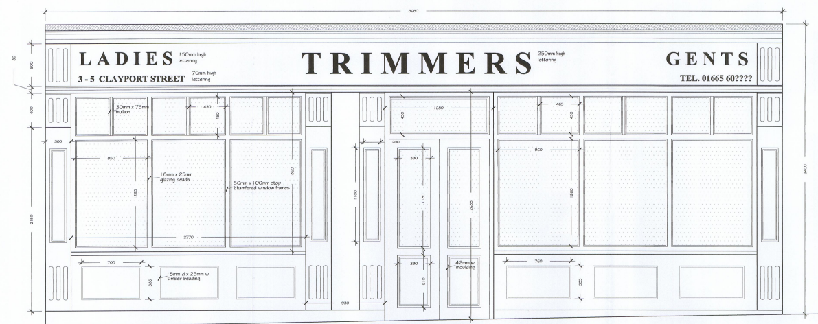
PROPOSED SHOP FRONT
