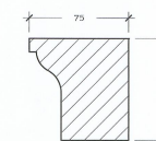
C/02 SECTION SCALE 1:2
