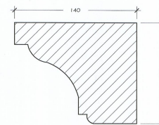
C/01 SECTION SCALE 1:2
